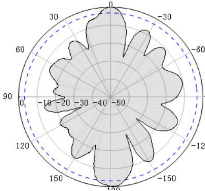
Vertical Beamwidth
