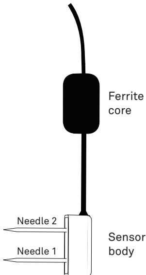
Figure 4 TEROS 10 sensor
